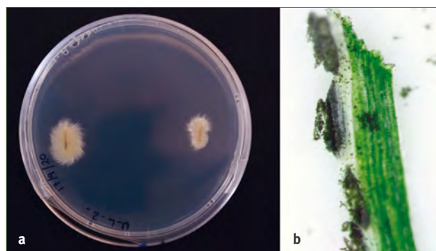
Koch's postulate testing for Ustilago sporoboli-indici following its inoculation onto Sporobolus laxus : a showing the recovered pathogen and b showing sori development typically found on plants infected with U. sporoboli-indici
