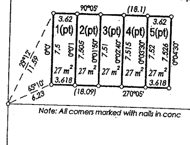
Figure 24.7: Illustrating a garage.
