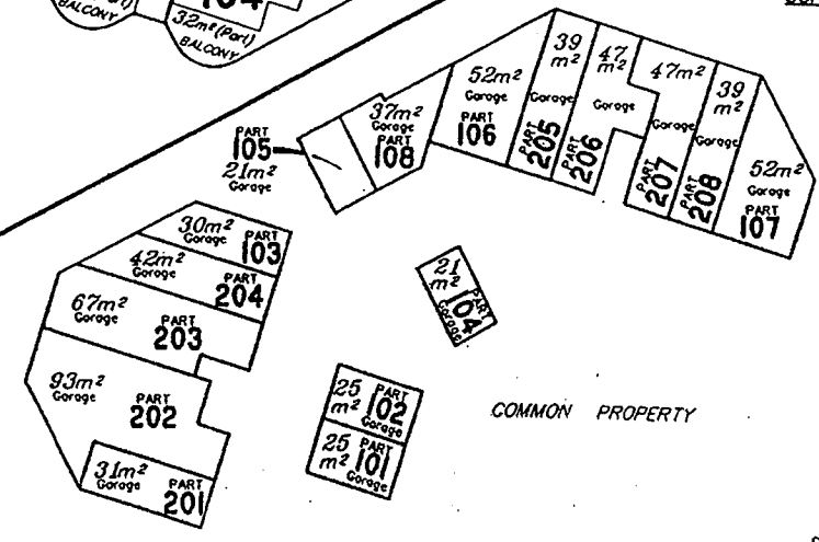
DIAGRAM A LEVEL A SCALE 1:300
